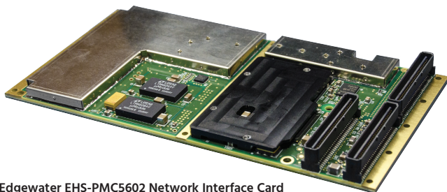
Edgewater EHS-PMC5602 Network Interface Card
