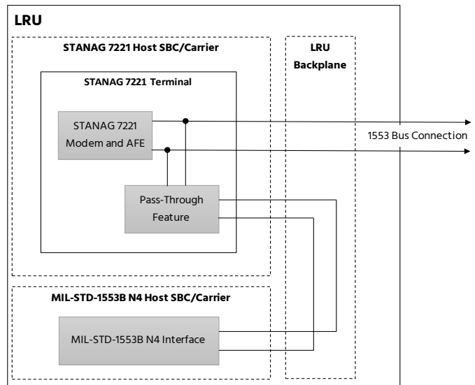
Figure 5: Legacy hookup through a Pass-Through Feature
