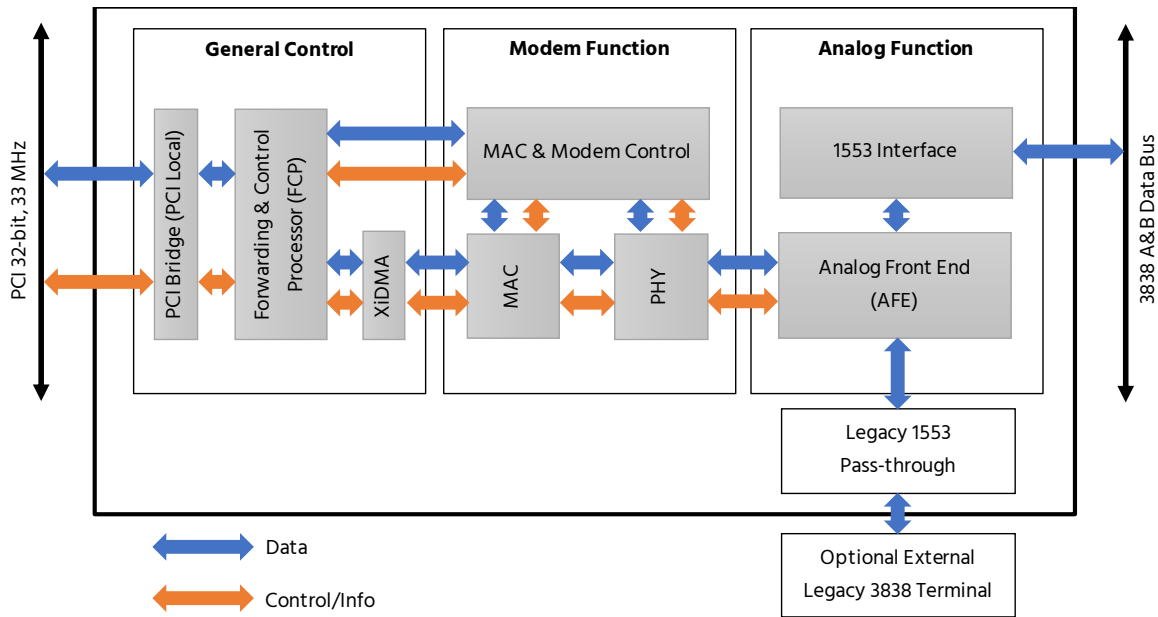
Figure 2: EHS-PMC6602 System Block Diagram
